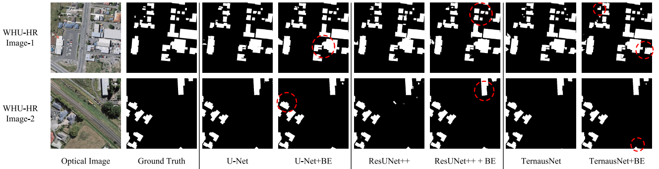
Fig. 8. Experimental result of the WHU-HR Dataset for each backbone network. The boundaries of building footprint are straightened and manifested, while adjacent buildings are distinguished well.
