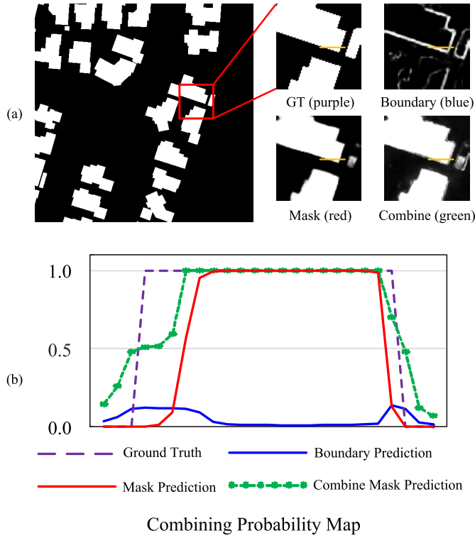
Fig. 3. (a) Predicted result of probability of boundary and mask. The predicted mask does not cover the ground truth sufficiently, and the predicted boundary can supplement the deficient area. The combining method is shown in (b), merging two probability maps for segmentation mask( P_m(x_m) ) and boundaries( P_b(x_b) ) expressed in yellow lines in (a). Missed pixel prediction of mask or irregular boundary of buildings can be supplemented by the combined probability map( P_s(x) ).
