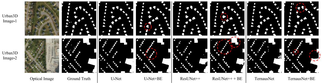
Fig. 7. Experimental result of the Urban 3-D Dataset for each backbone network. The boundaries of building footprint are straightened and manifested, while adjacent buildings are distinguished well.
