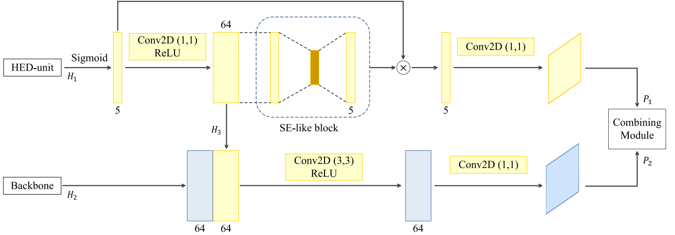
Fig. 2. Structure of the BE module. H_1 is the concatenated output of the HED unit containing boundary information. H_2 is the segmentation mask produced by the backbone network. Both H_1 and H_2 are adopted to subunits of the BE module in parallel. Two parallel subunits extract and enhance both boundary and segmentation masks, producing each probability map P_1 and P_2 . The two probability maps will be integrated by combining probability map & positive replacement .
