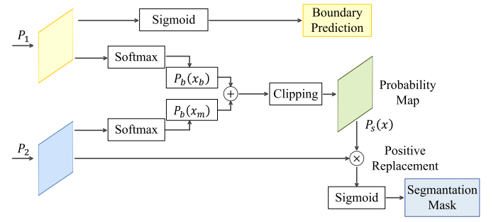
Fig. 4. Combining module consists of probability map and positive replacement. The probability map enhances the edge of segmentation mask directly, and the combined result will replace the original segmentation mask maintaining its scale by positive replacement.
