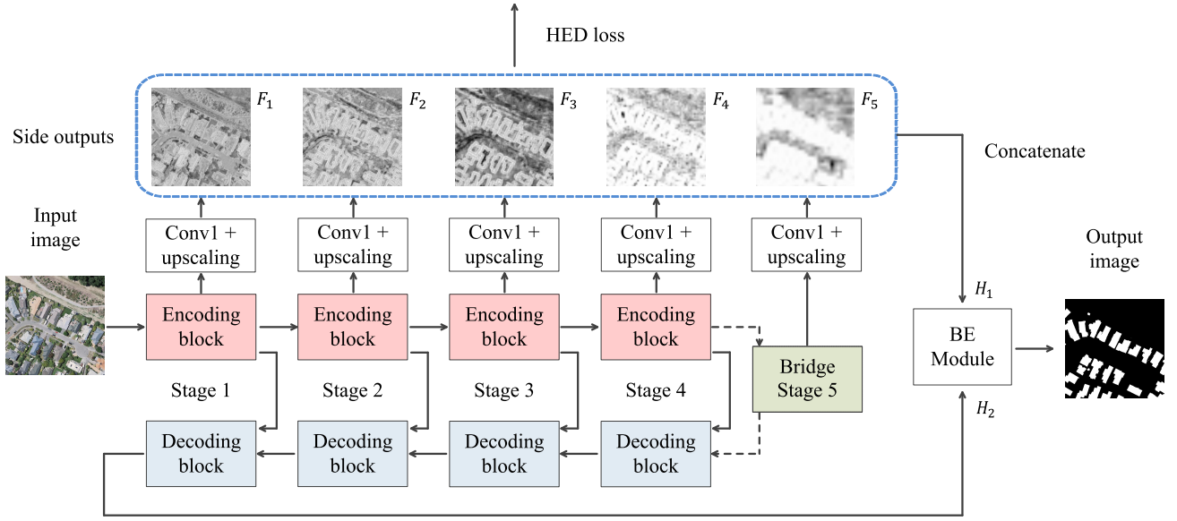
Fig. 1. HED unit is attached to a given backbone's encoder. The side outputs are extracted from the last feature maps in each stage being stretched as the same size as the input shape. The side outputs become an auxiliary prediction to guide the network to detect edges of the target object as being corrected by HED loss, L_{HED} . Consequently, the concatenated side outputs will be input to the BE module. Although this figure is an example based on U-Net, the HED unit can be applied to any backbone containing the encoder-decoder architecture.
