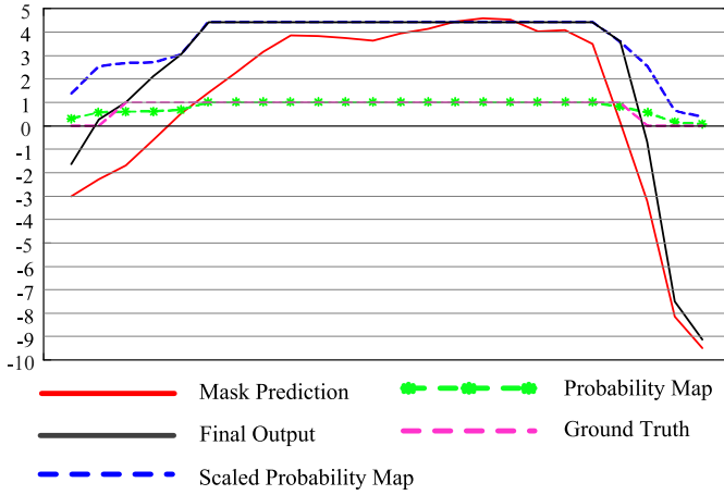
Fig. 5. Raw signal values of the mask prediction ( x_m ) are modified by the combined probability map ( P_s(x) ). Positive signals ( \sigma(x_m) ) in x_m are removed and replaced with the scaled combined probability map ( P_s(x)\lambda(x_m) ), while the negative signals are supplemented. The adjusted prediction, final output ( x_{\text{output}} ), shows improved results fitting well with the ground truth.
